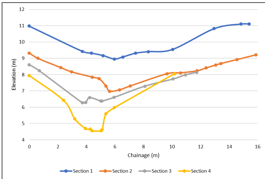
Figure 3: Cross-Section Profiles
